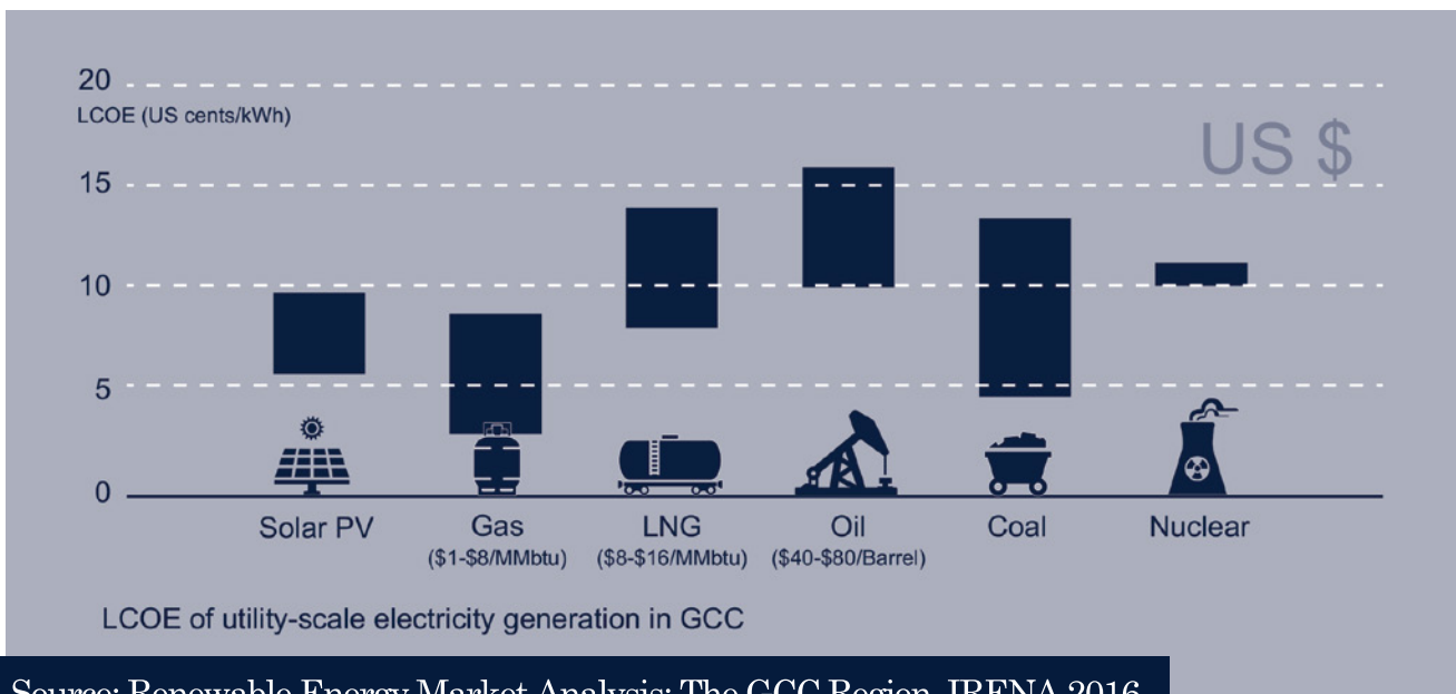
Figure 5: Solar PV in GCC can be cost competitive with electricity from oil and LNG at Current prices.
